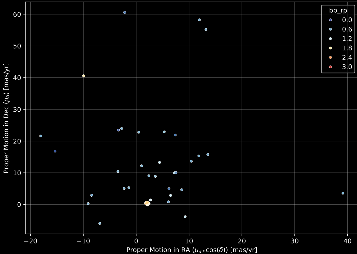
APOGEE DR17 Field: [LMC8] Proper Motion Diagram (n= 109)
