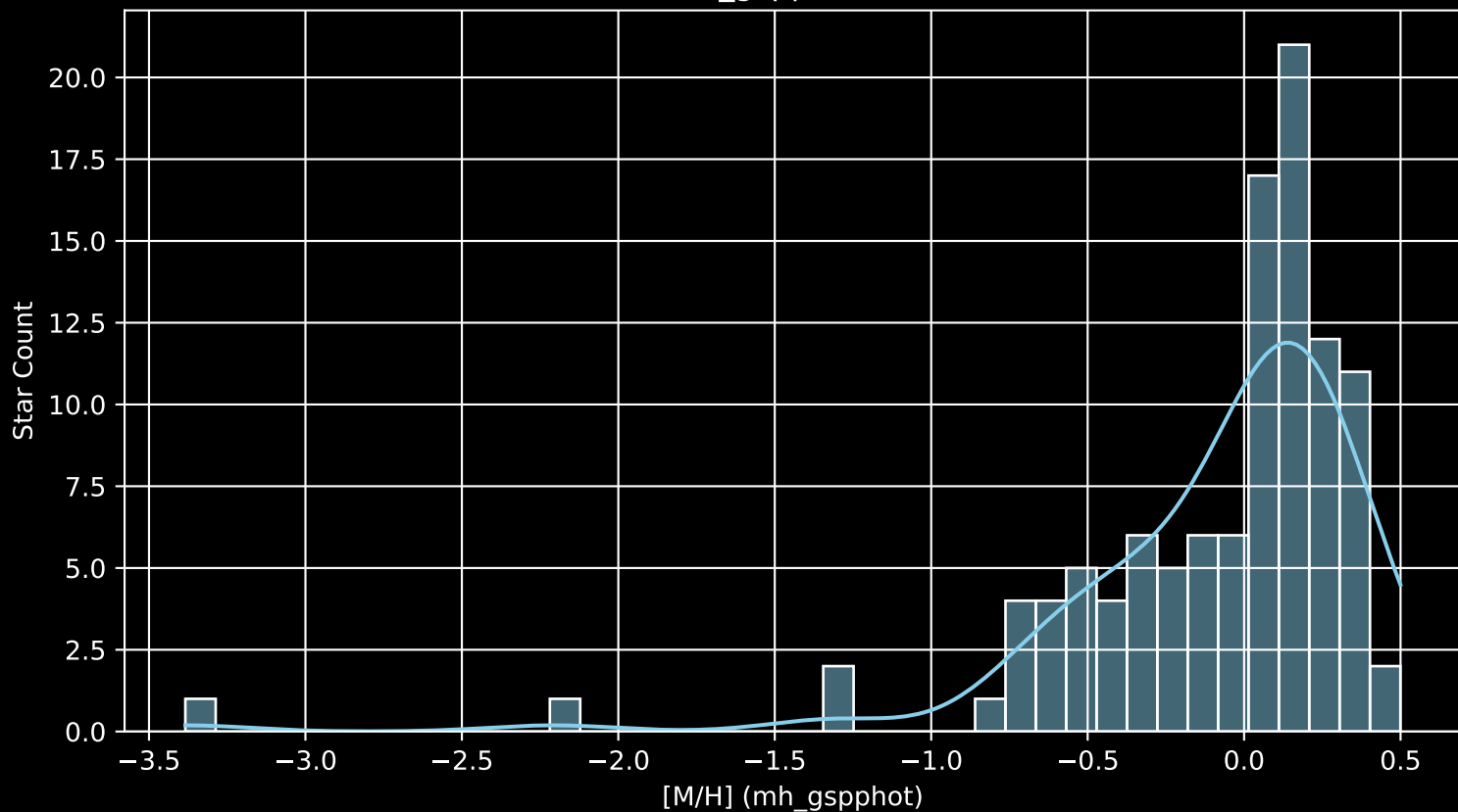
APOGEE DR17 Field: [LMC8 [M/H] (mh_gspphot) (n= 108)
