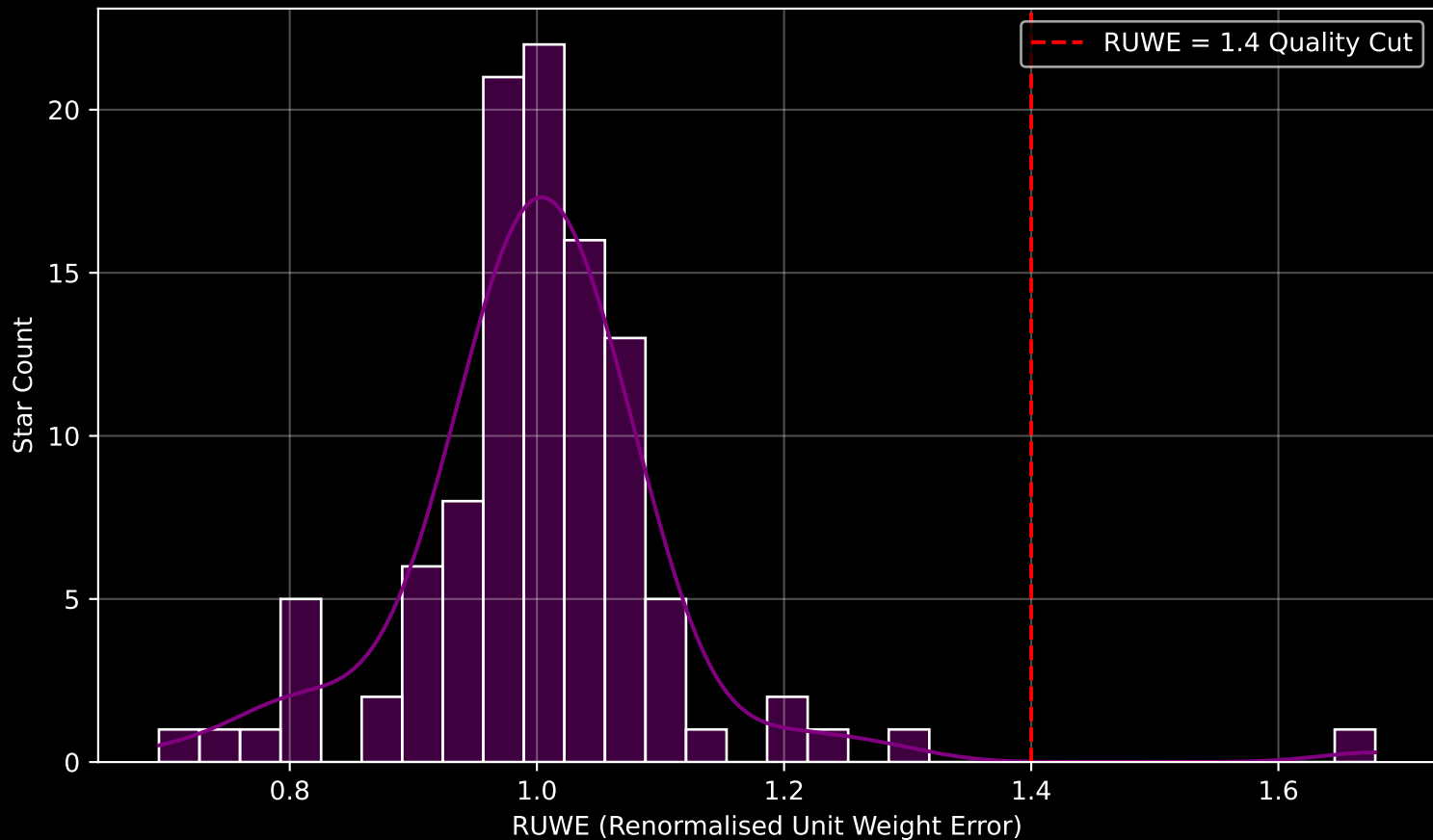
GAPOGEE DR17 Field [LMC8] RUWE Distribution (n= 107)
