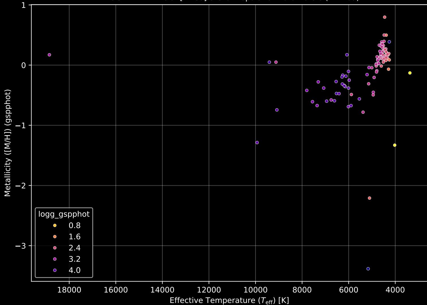
APOGEE DR17 Field: [LMC8] Stellar Population Parameters (n= 109)
