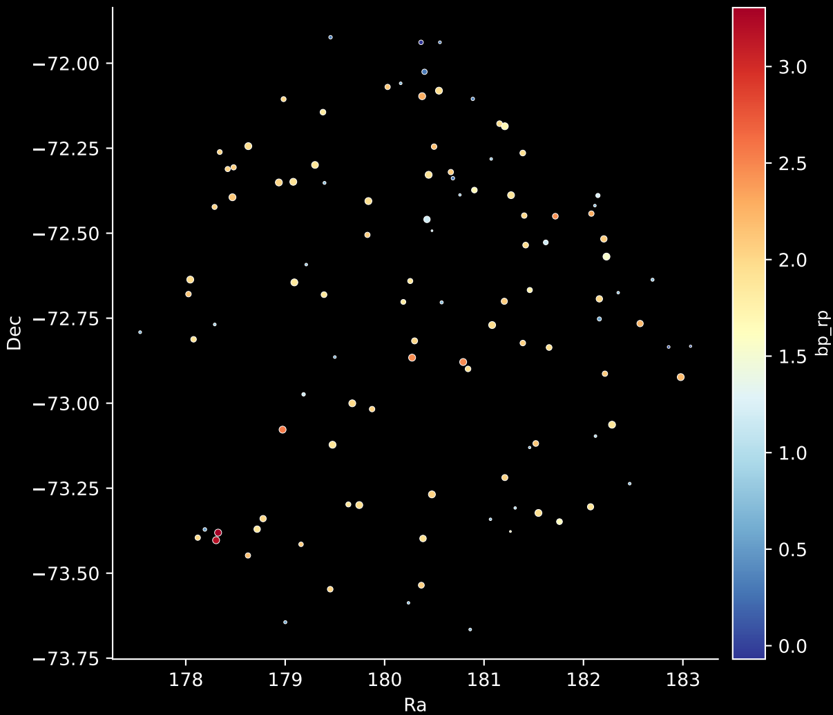
APOGEE DR17 Field: [LMC8] Stars: 109
