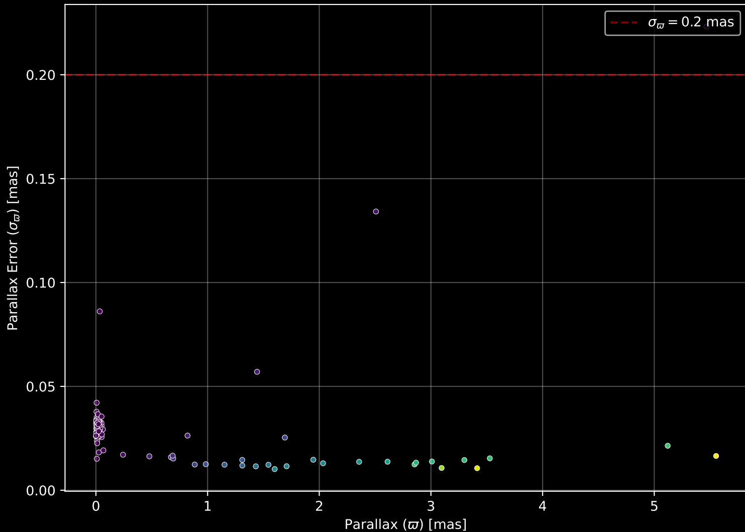
APOGEE DR17 Field: [LMC8] Parallax Quality (n= 109)
