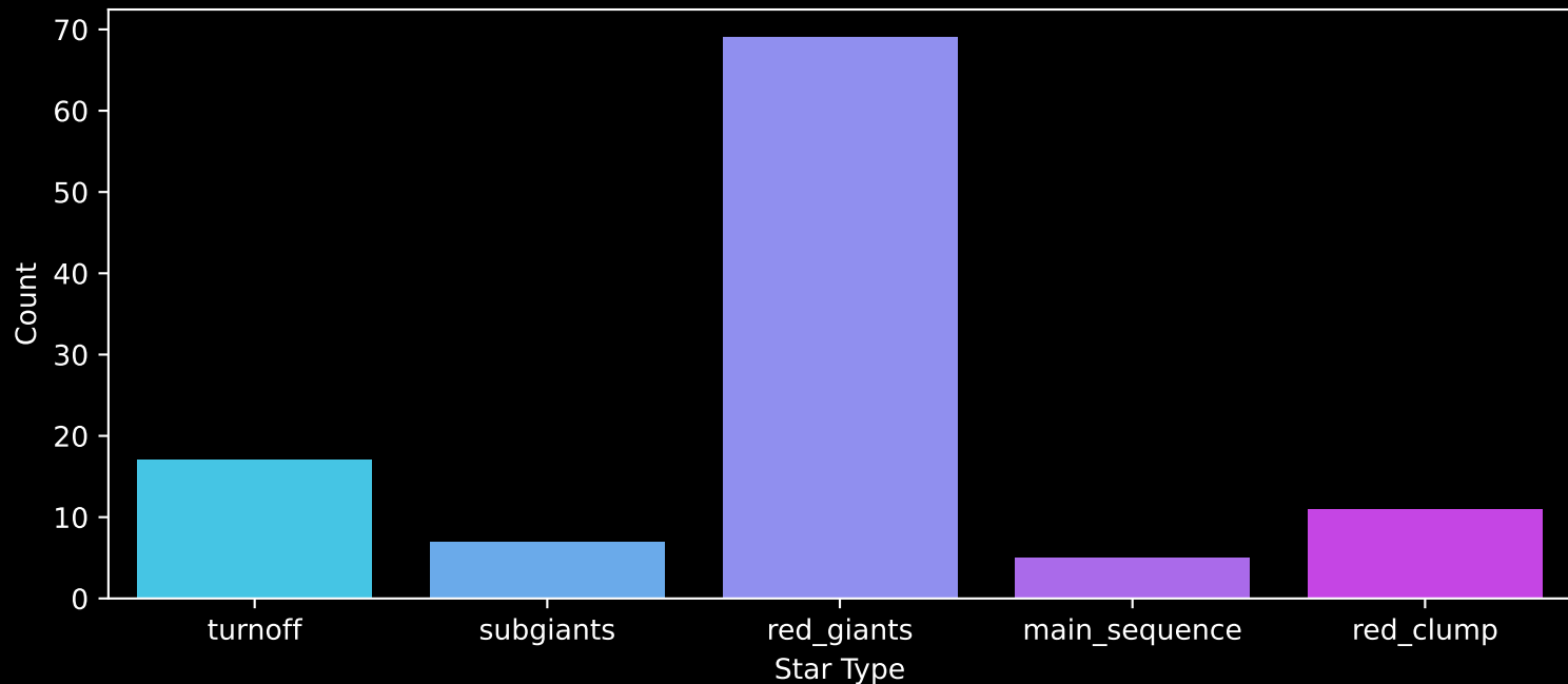
APOGEE DR17 Field: [LMC8] Count plot of Star Type
